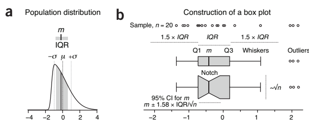
Figure 1 | The construction of a box plot. (a) The median ( m = -0.19 , solid vertical line) and interquartile range ( IQR = 1.38 , gray shading) are ideal for characterizing asymmetric or irregularly shaped distributions. A skewed normal distribution is shown with mean \mu = 0 (dark dotted line) and s.d. \sigma = 1 (light dotted lines). (b) Box plots for an n = 20 sample from a. The box bounds the IQR divided by the median, and Tukey-style whiskers extend to a maximum of 1.5 \times IQR beyond the box. The box width may be scaled by \sqrt{n} , and a notch may be added approximating a 95% confidence interval (CI) for the median. Open circles are sample data points. Dotted lines indicate the lengths or widths of annotated features.
